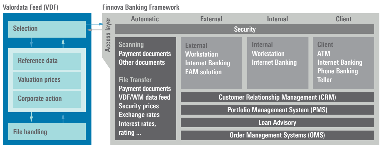
Connection between SIX Financial Information's data offering and Finnova Banking Framework.
